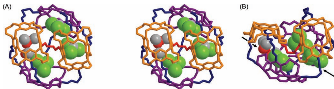
Figure 1. Stereo view of a tube model of the X-ray structure of nanocapsule 1a \text{O}[\text{CHCl}_2]_3[\text{CH}_3\text{OH}]_3 along the pseudo - C_2 axis (A) and view perpendicular to it (B). Appending pentyl groups, hydrogen atoms, and second component of disordered groups are omitted for clarity. Solvent molecules inside the cavity of 1a are shown as space-filling models. Pairs of symmetry-related cavitands are colored in purple and orange. \text{CH}=\text{N}-\text{CH}_2\text{CH}_2-\text{N}=\text{CH} linkers are colored blue and red. Openings to the two cavities of 1a are marked with arrows in (B).
