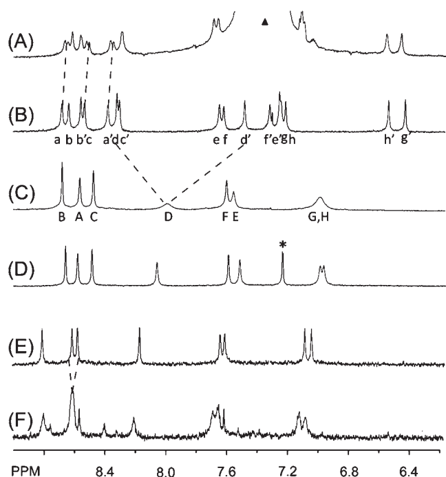
Figure 2. Partial ^1\text{H} NMR spectra (400 MHz) of 1a showing the imine and aryl proton region of the spectrum. At -30\text{ }^\circ\text{C} in \text{CD}_2\text{Cl}_2 + 2.7\% (v/v) (-) - S -1-phenylethanol (A) and in \text{CD}_2\text{Cl}_2 (B). At 60\text{ }^\circ\text{C} in \text{CD}_2\text{Cl}_2 (C), \text{CDCl}_3 (D) and \text{CDCl}_2\text{CDCl}_2 (E). At 110\text{ }^\circ\text{C} in \text{CDCl}_2\text{CDCl}_2 (F). Signals assigned to imine and aryl protons of 1a , \text{CHCl}_3 and (-) - S -1-phenylethanol are marked with letters a–d, e–h, asterisk, and filled triangle, respectively.
